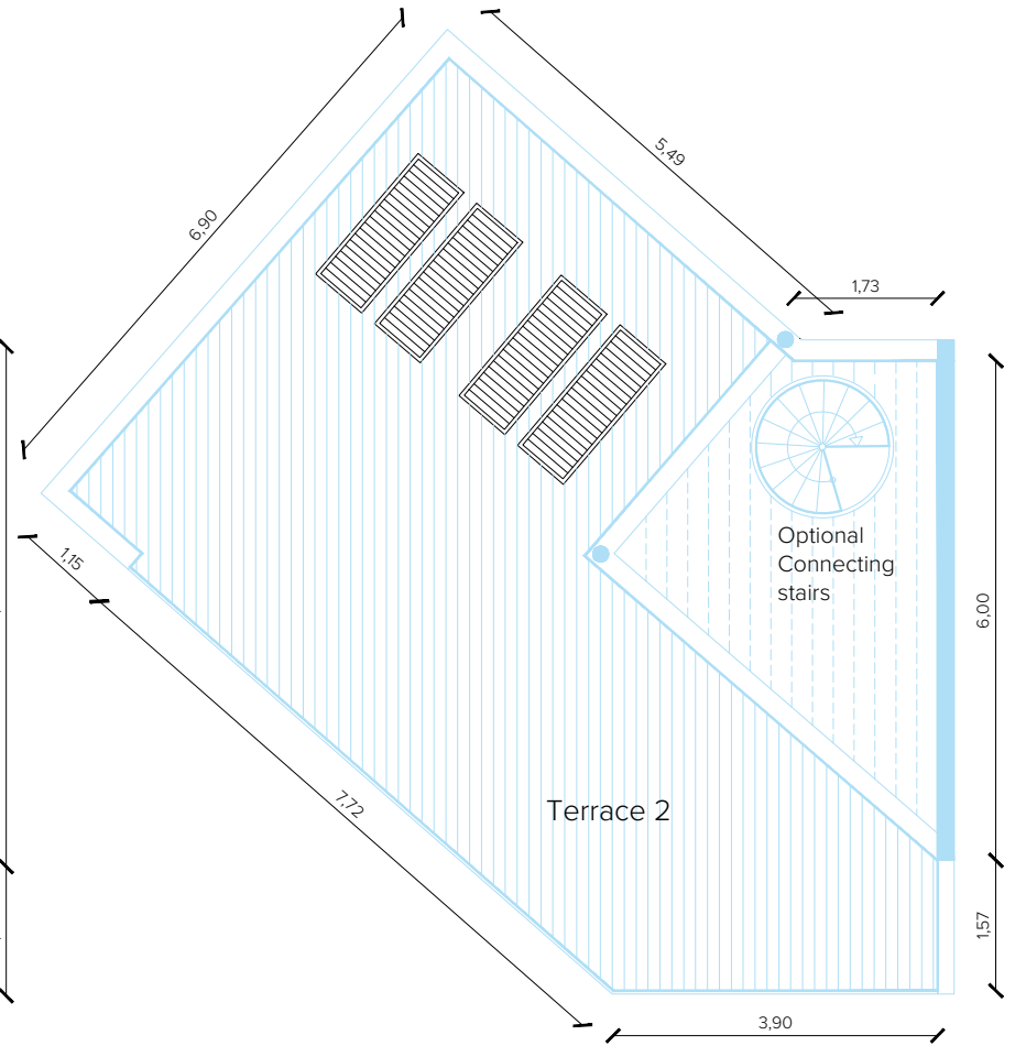
TERRACE PLAN
